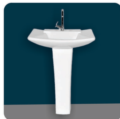
1016 Wash Basin Pedestal Size : W 485 L 600 H 180mm Pedestal : 690mm (27")
