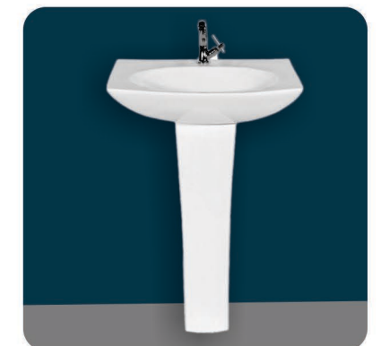
1015 Wash Basin Pedestal Size : W 485 L 590 H 175mm Pedestal : 690mm (27")
