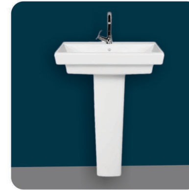
1009 Wash Basin Pedestal Size : W 445 L 580 H 150mm Pedestal : 690mm (27")
